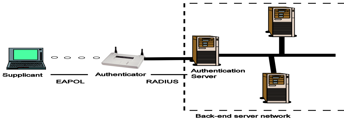
Figure 8: IEEE 802.1x in 802.11 WLANs
