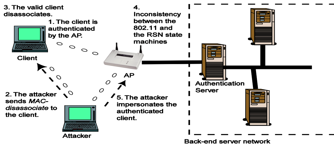
Figure 10. Session Hijack Attack in 802.11i
